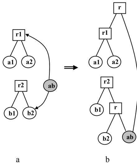
Figure 6. Merging of two DTs.
