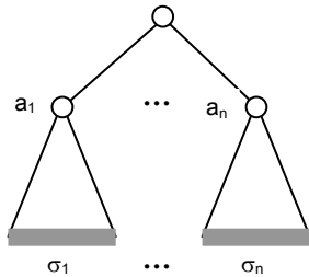
Figure 2. Adjacency of siblings is reflected as adjacency of covered spans.
