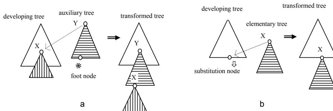
Figure 1. Adjunction (a) and substitution (b).
