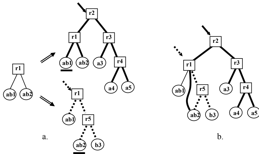
Figure 7. Splitting a DT onto two separate threads.
