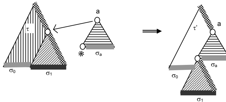
Figure 4. Adjunction of a left-footed AT on the RF of the DT.
