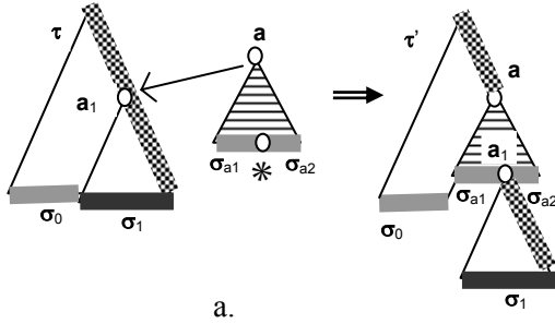
Figure 5. Cases that result in violation of the SP.
